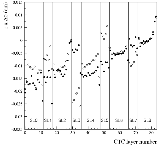
FIG. 7. The deviation ( r \times \Delta\phi ) of each CTC layer from its nominal position at the end plates ( |z| = 150 \text{ cm} ) in cm, versus the layer number. The solid (open) circles represent the west (east) CTC end plate.
