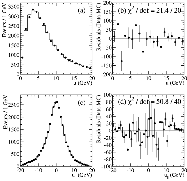
FIG. 37. The (a) |u| and (c) u_{\parallel} distribution distribution for the W \rightarrow e \nu sample. The points (histograms) are the data (simulation). The differences between the data and the simulation are shown in (b) and (d).
