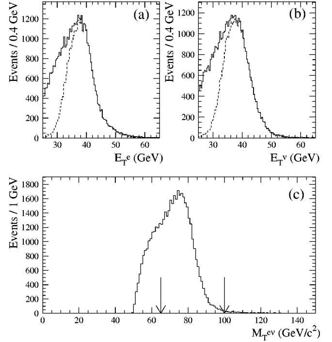
FIG. 16. Kinematic quantities from the final W \rightarrow e\nu sample. E_T distributions of (a) electrons and (b) neutrinos. The dashed curves show the events in 65 < M_T < 100 GeV, the fit region for the W mass measurement. (c) Transverse mass distribution. The arrows indicate the region used in the W mass fit.
