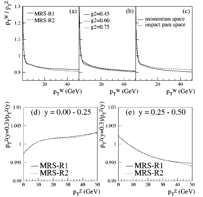
FIG. 26. The ratios of the p_T^W to p_T^Z distribution from resummed calculations in impact parameter space showing (a) PDF dependence, and (b) nonperturbative parameter dependence. The ratios in impact parameter space and p_T space are compared in (c). The ratio of p_T^Z at y^Z=0.3 to p_T^Z for (d) 0 < y^Z < 0.25 , and (e) 0.25 < y^Z < 0.5 .
