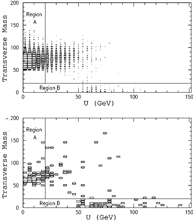
FIG. 22. M_T ( \text{GeV}/c^2 ) vs |u| distributions without M_T and |u| cuts for all W data (top), and a QCD subset of the W data (bottom).
