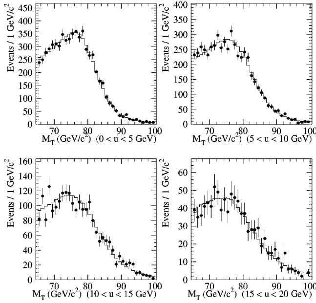
FIG. 52. Transverse mass distributions in bins of |u| for the W \rightarrow \mu\nu data (points) and the best fit simulation (histograms). The four |u| bins are 0 < |u| < 5 GeV (top left), 5 < |u| < 10 GeV (top right), 10 < |u| < 15 GeV (bottom left), and 15 < |u| < 20 GeV (bottom right).
