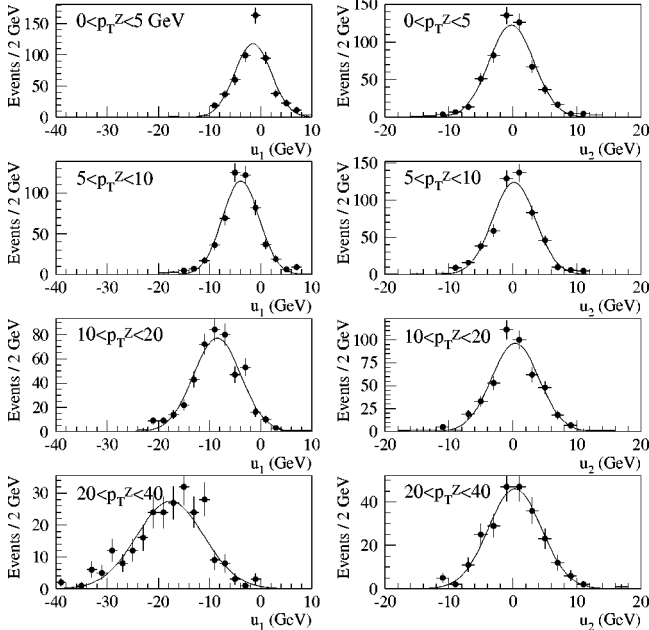
FIG. 32. The fit of the u_1 and u_2 distributions in ranges of Z p_T in the muon sample, illustrating the adequacy of assuming Gaussian resolution (solid lines).
