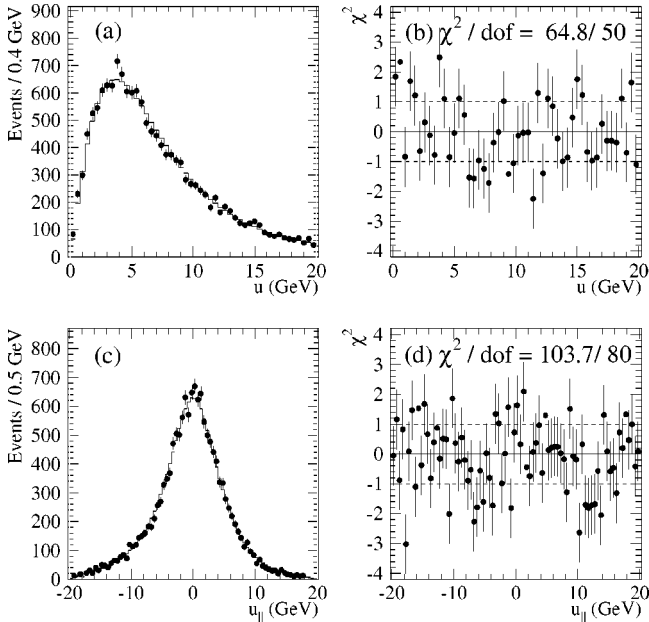
FIG. 38. The (a) |u| and (c) u_{\parallel} distribution distribution for the W \rightarrow \mu \nu sample. The points (histograms) are the data (simulation). The differences between the data and the simulation normalized by the statistical uncertainty are shown in (b) and (d).
