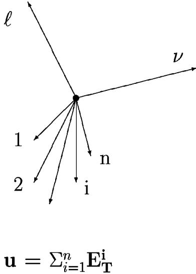
FIG. 2. Kinematics of W boson production and decay for the events used in this analysis, as viewed in the plane transverse to the antiproton-proton beams. The recoil energy vector \mathbf{u} is the sum of the transverse energy vectors \mathbf{E}_T^i of the particles recoiling against the W . Although energy is a scalar quantity, “transverse energy” commonly denotes the transverse component of the vector whose magnitude is the energy of the particle and direction is parallel to the momentum of the particle.
