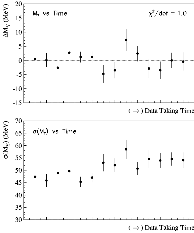
FIG. 13. Variation of the measured Y(1S) mass (top) and width (bottom) as a function of time. The left side of the plot corresponds to January 1994 and the right side of the plot to July 1995. \Delta M_Y is difference between the measured mass for a given time period and the mass using all the data.
