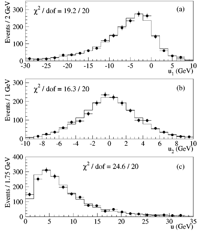
FIG. 33. (a) u_1 , (b) u_2 , and (c) |\mathbf{u}| distributions for the Z \rightarrow \mu^+ \mu^- data. The histograms are the simulation using the recoil model parameters.
