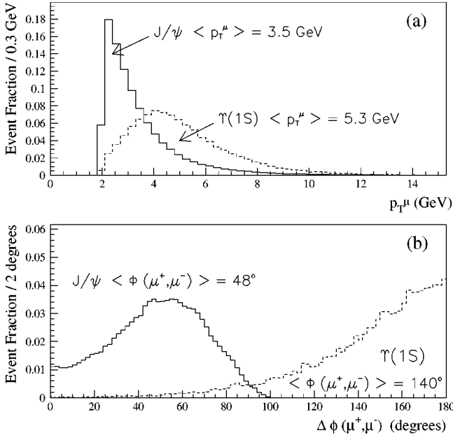
FIG. 10. (a) Transverse momentum distributions of muons and (b) opening angle distributions between \mu^+ and \mu^- in the \Upsilon(1S) and J/\psi samples. The histograms are normalized to unit area.
