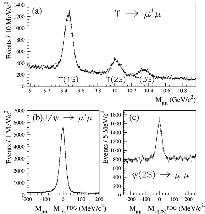
FIG. 12. The measured dimuon mass spectra near the (a) Y masses, (b) J/\psi mass, and (c) \psi(2S) mass. The curves are the best fits of line shapes from the Monte Carlo simulation.
